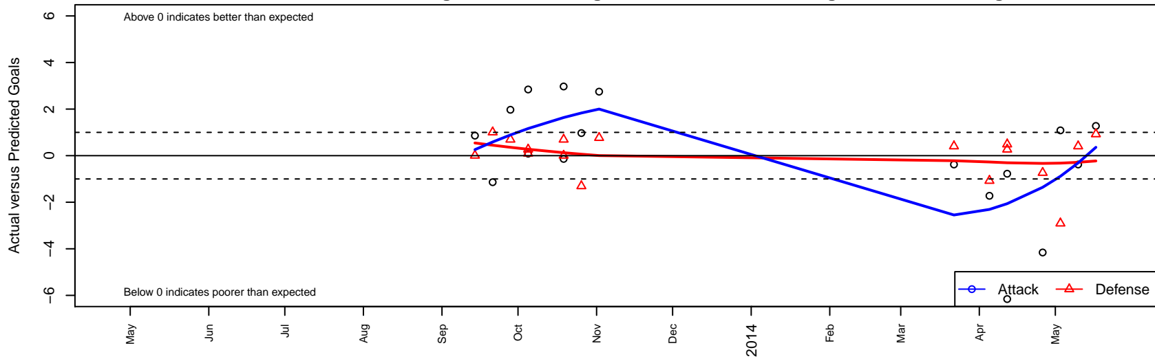
Columbia Basin YSA Extreme G99 Dots are actual minus expected GF (blue circles) and GA (red triangles). Blue line is smoothed change in attack strength. Red is smoothed change in defense strength.
